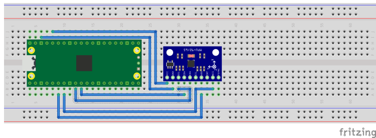
Figure 12. Wiring Diagram for MPU9250.
