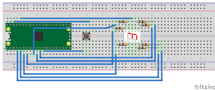
Figure 8. Wiring Diagram for 7 segment LED.
