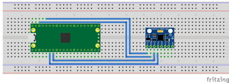
Figure 13. Wiring Diagram for MPU6050.
