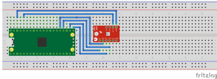
Figure 11. Wiring Diagram for bme280.
